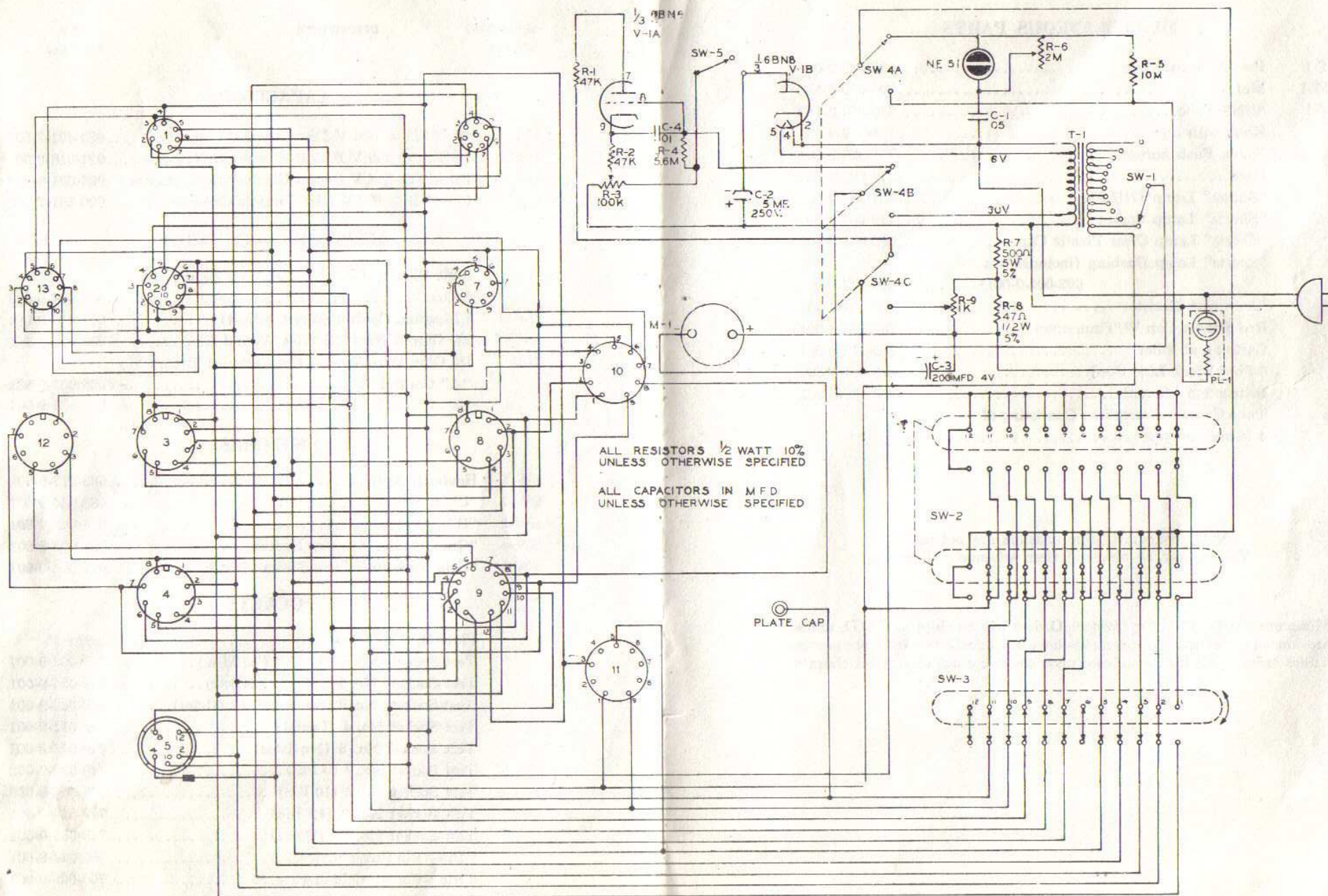
B & K MFG. CO. MODEL 606 TUBE TESTER
